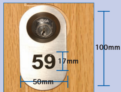
RFM NP2 Oval with 23mm hole and 17mm text
