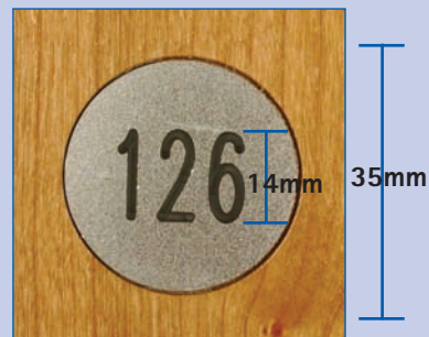
RFM NP6 35mm round plastic number
